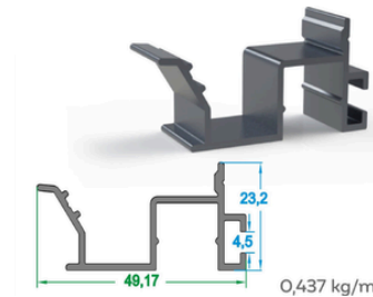
Yan Oluk Kapak Profili Side Gutter Cover Profile
