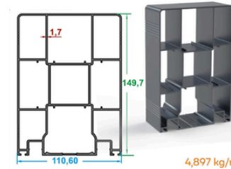
110'luk Işıklı Ray Profili 110 Light Rail Profile
