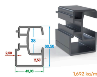
Küçük Ray Profili Small Rail Profile
