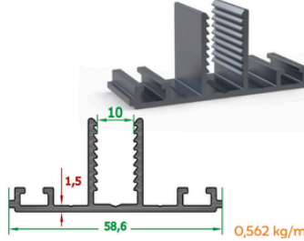
Cam Alt Baskı Profili Glass Holder Profile
