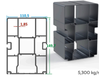
Yandan Kanallı 110'luk Ray Profili Side Channel 110 Rail Profile
