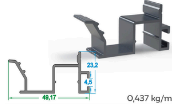
Yan Oluk Kapak Profili Side Gutter Cover Profile
